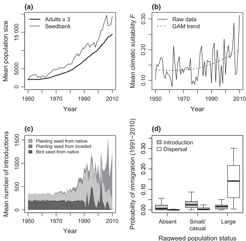
Fig. 4 The modelled ragweed invasion is driven by climate and trade. (a) Modelled relative population growth of adults and the seed-bank, averaged over the 0.5% top model parameterizations. (b) Time series of the mean fecundity index in the modelled region from the top parameterizations, showing a significant increase in climatic suitability over time (generalized additive model [GAM], P = 0.004 , R^2 = 0.188 ). (c) Stacked time series of simulated introductions by all trade pathways, where shaded areas represent the numbers of introduction. (d) Boxplots of the average annual modelled probabilities of introduction from all trade pathways and neighbourhood seed dispersal into a grid cell with different population statuses (see Fig. 2). Outlying observations are omitted for clarity.
